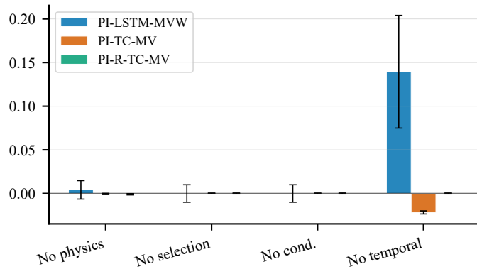
IEEE 30 bus (DC)
