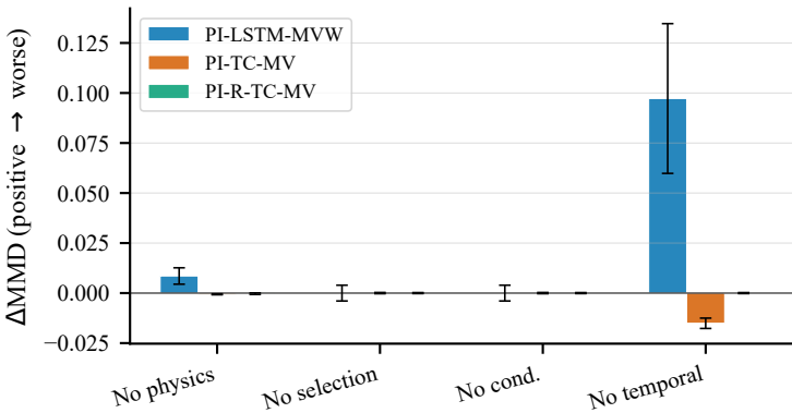
IEEE 14 bus (DC)
